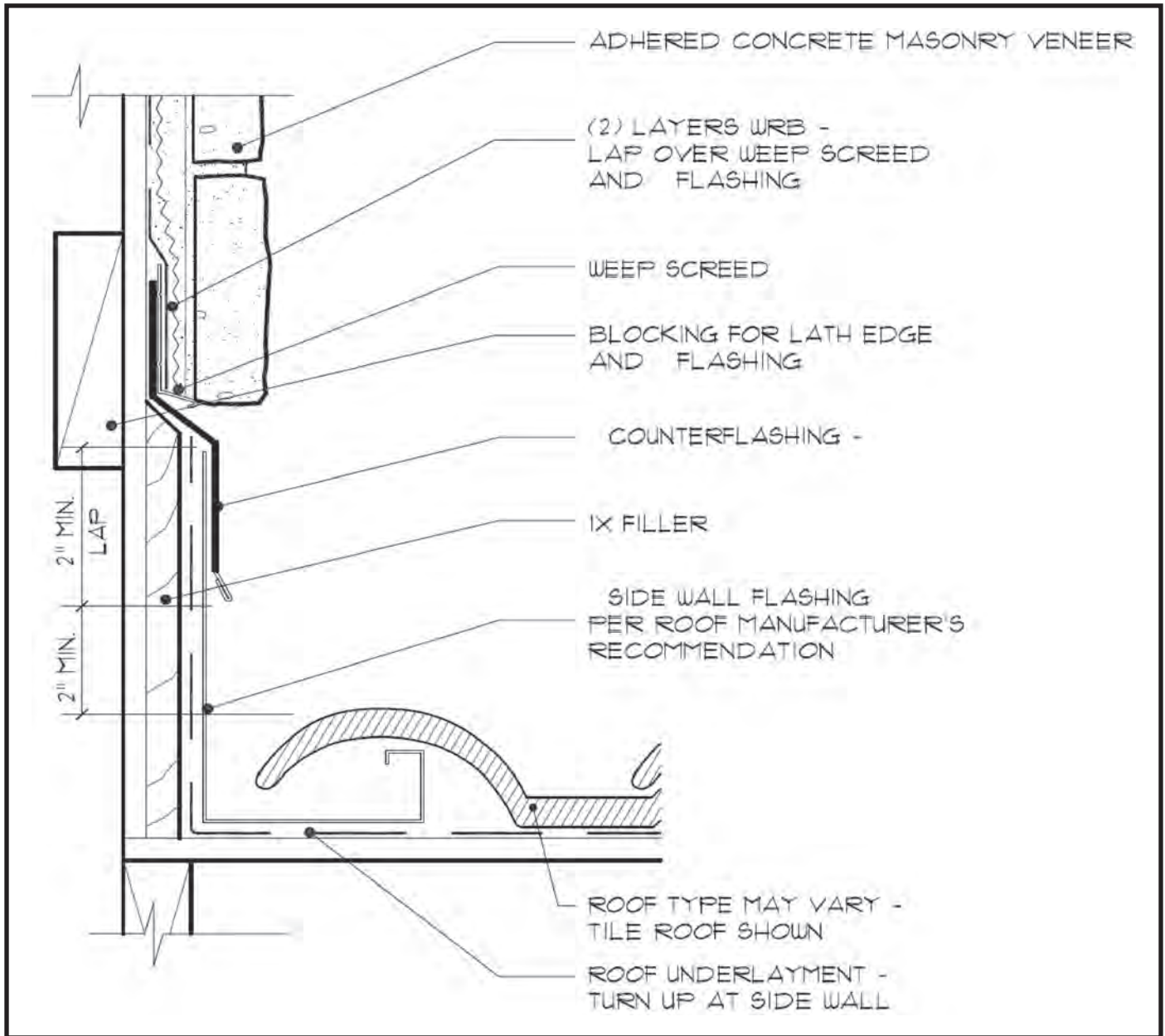
Fig. 18. Side Wall - Tile Roofing Curbing
