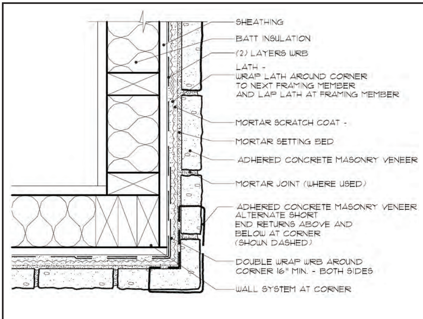
Fig. 7. Outside Corner
