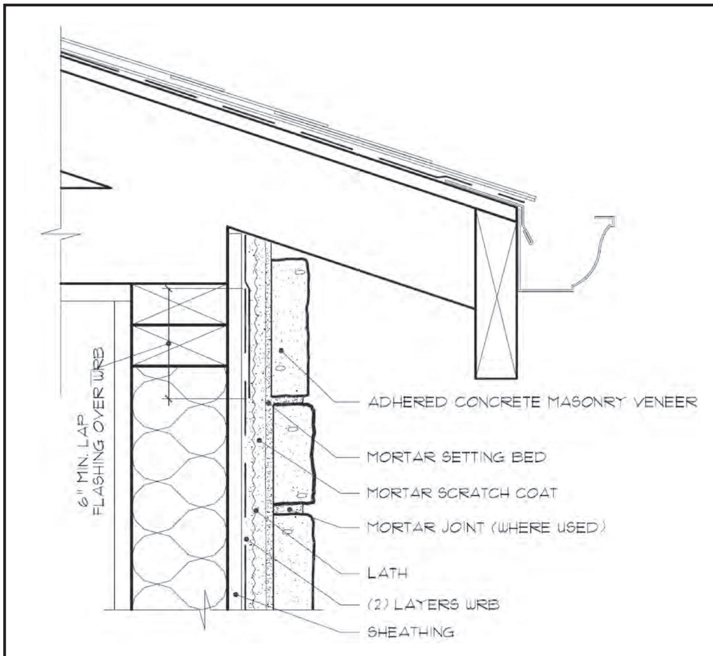
Fig. 11. Open Eave - Overhang
