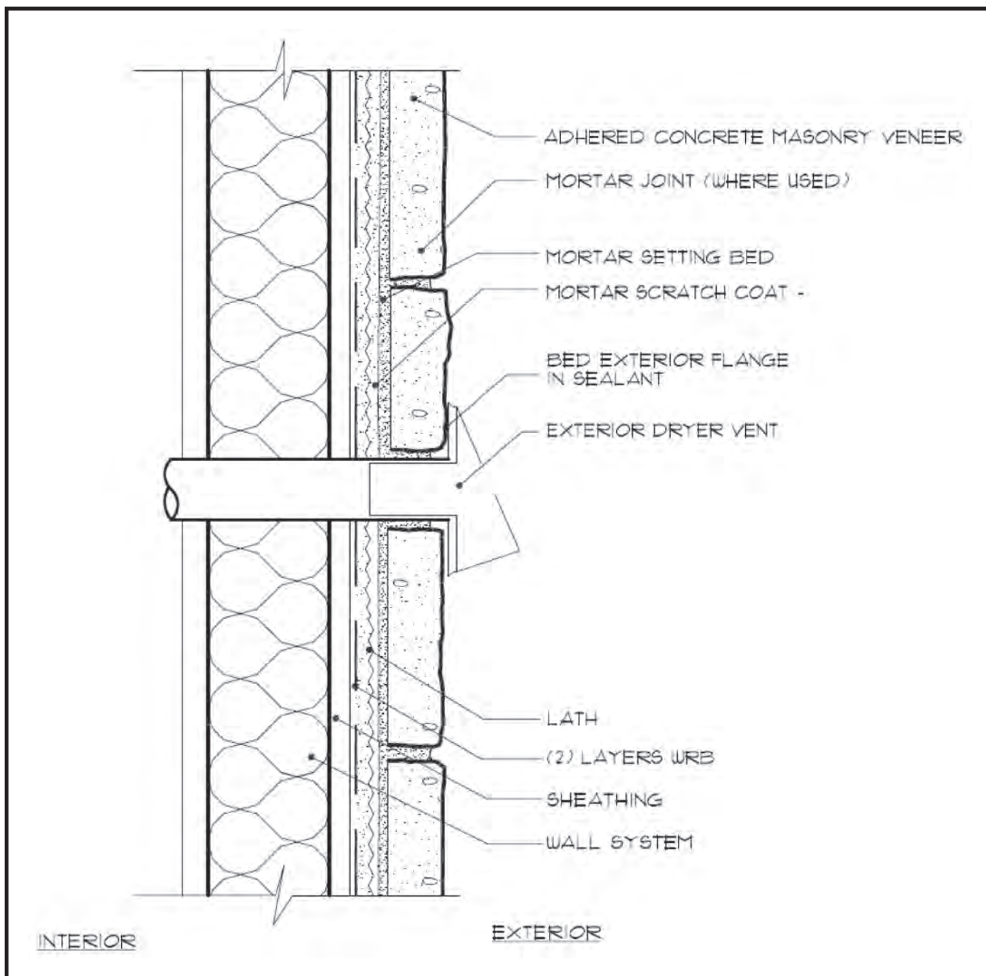
Fig. 29. Dryer Vent Penetration
