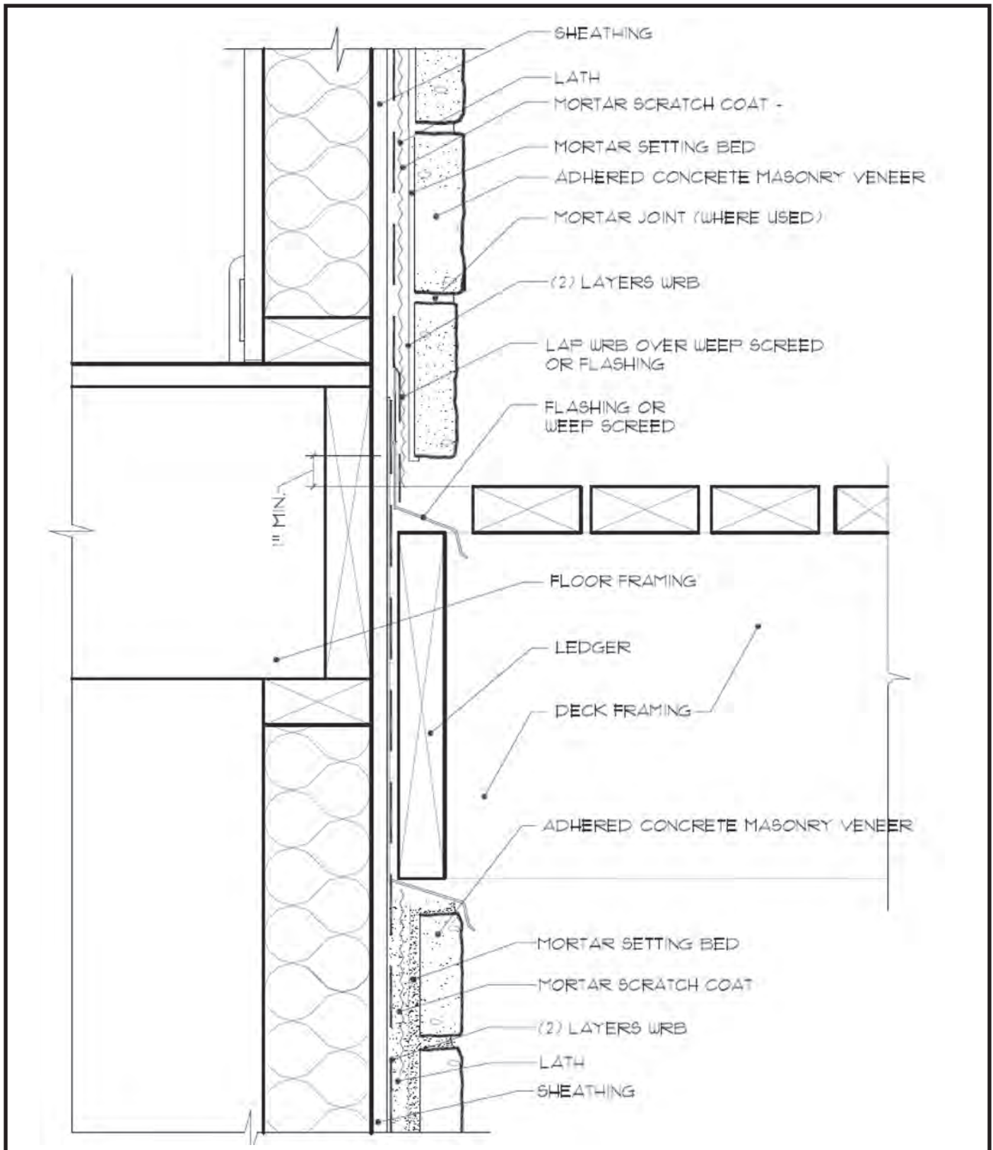
Fig. 30. Deck Termination
