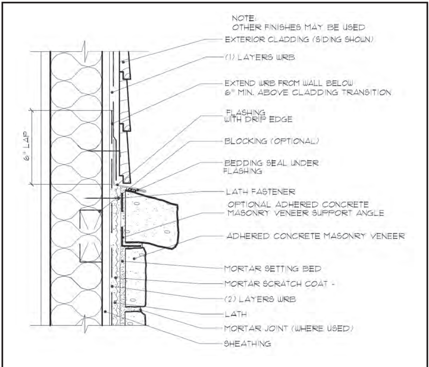
Fig. 6. Cladding Transition
