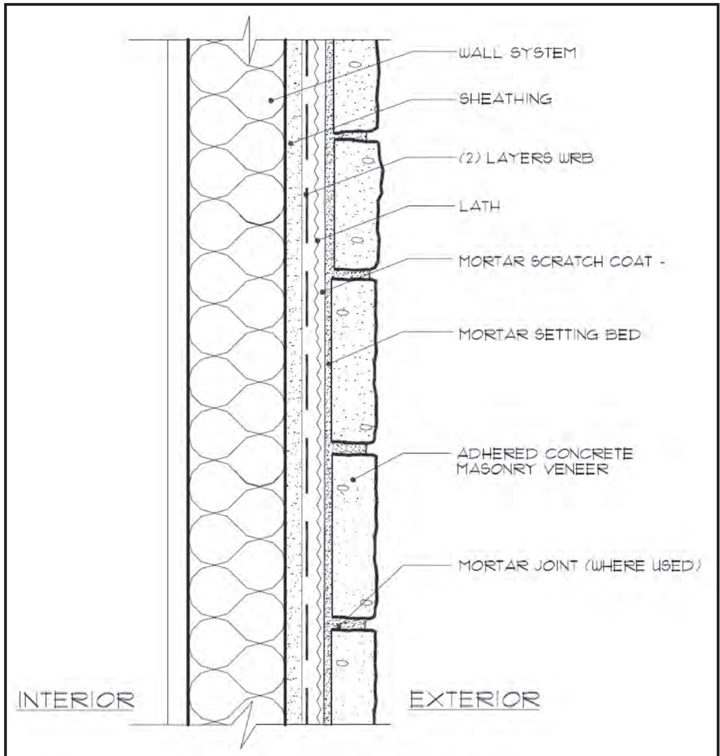
Fig. 2. Typical Wall Section
