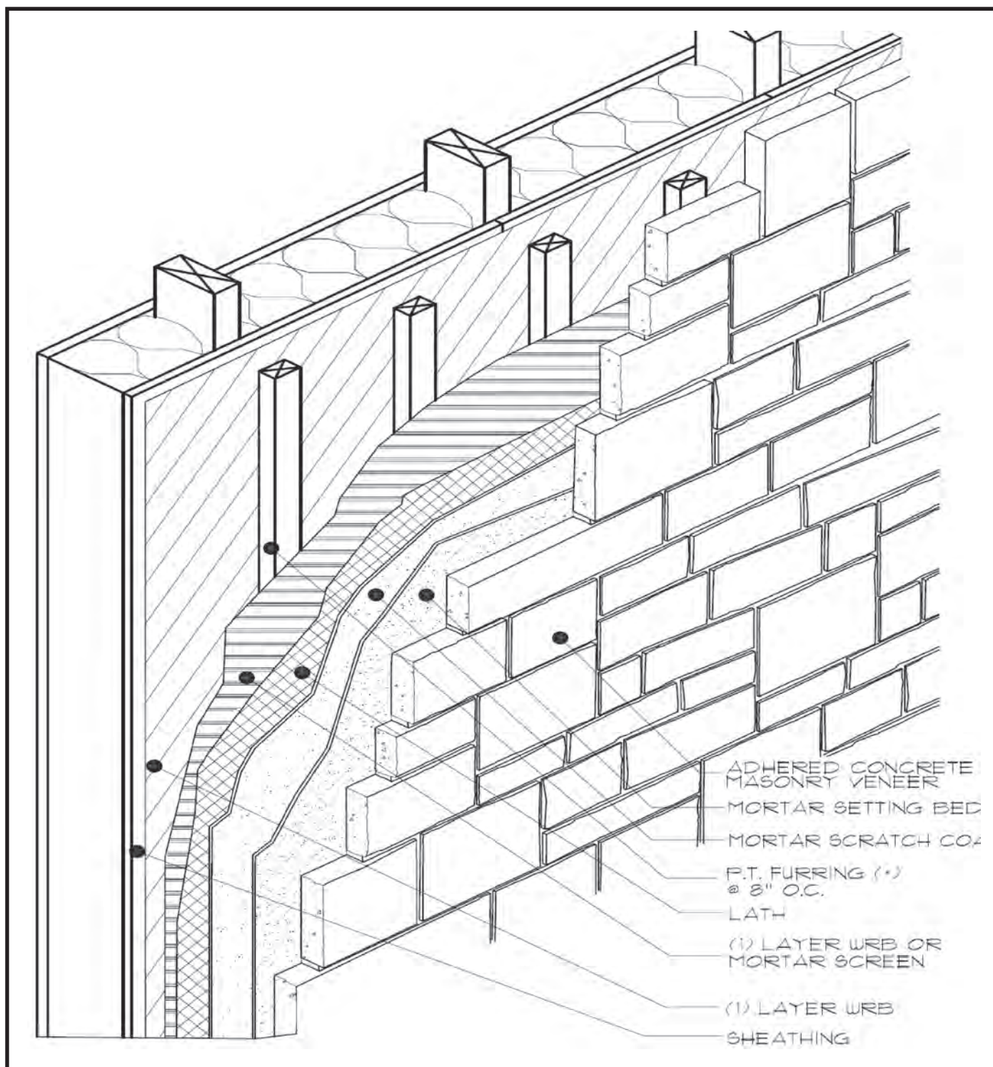
Fig. 33. Wall Assembly - Optional Rainscreen System - Strapped
