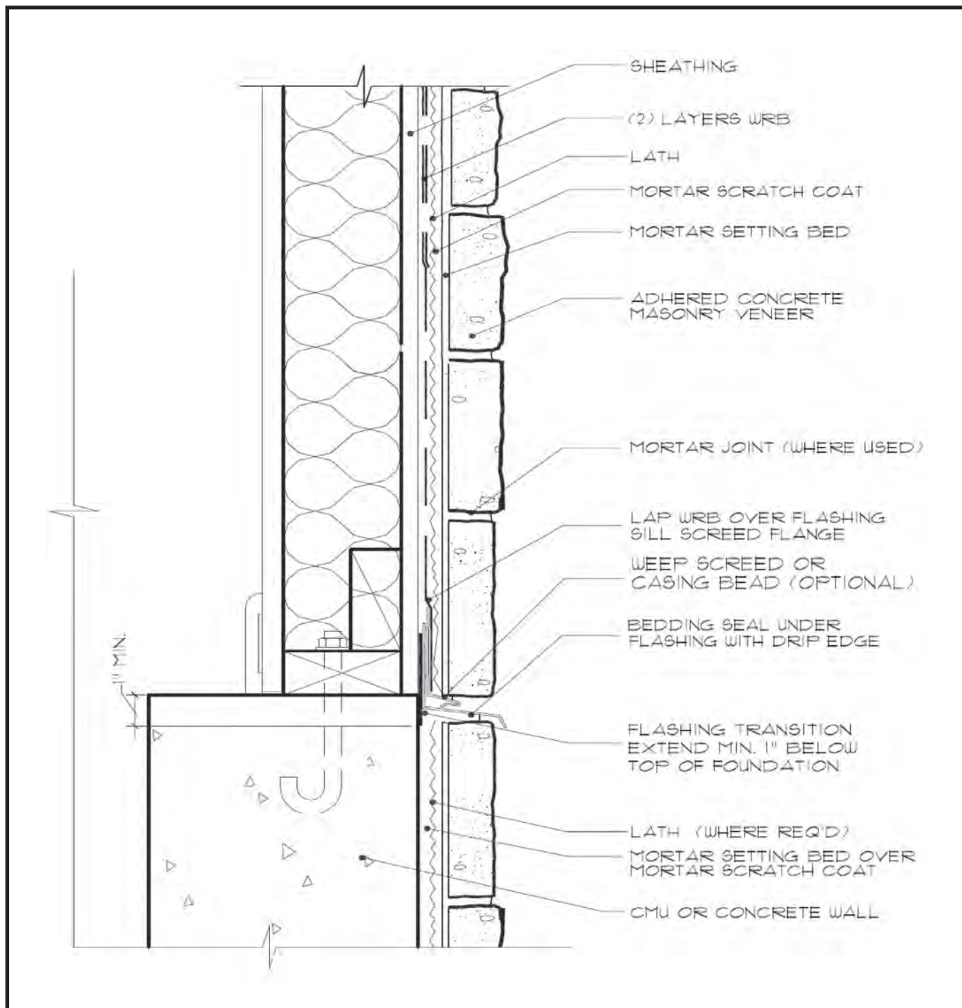
Fig. 5. Foundation Wall - Transition to ACMV Continuing Down Foundation
