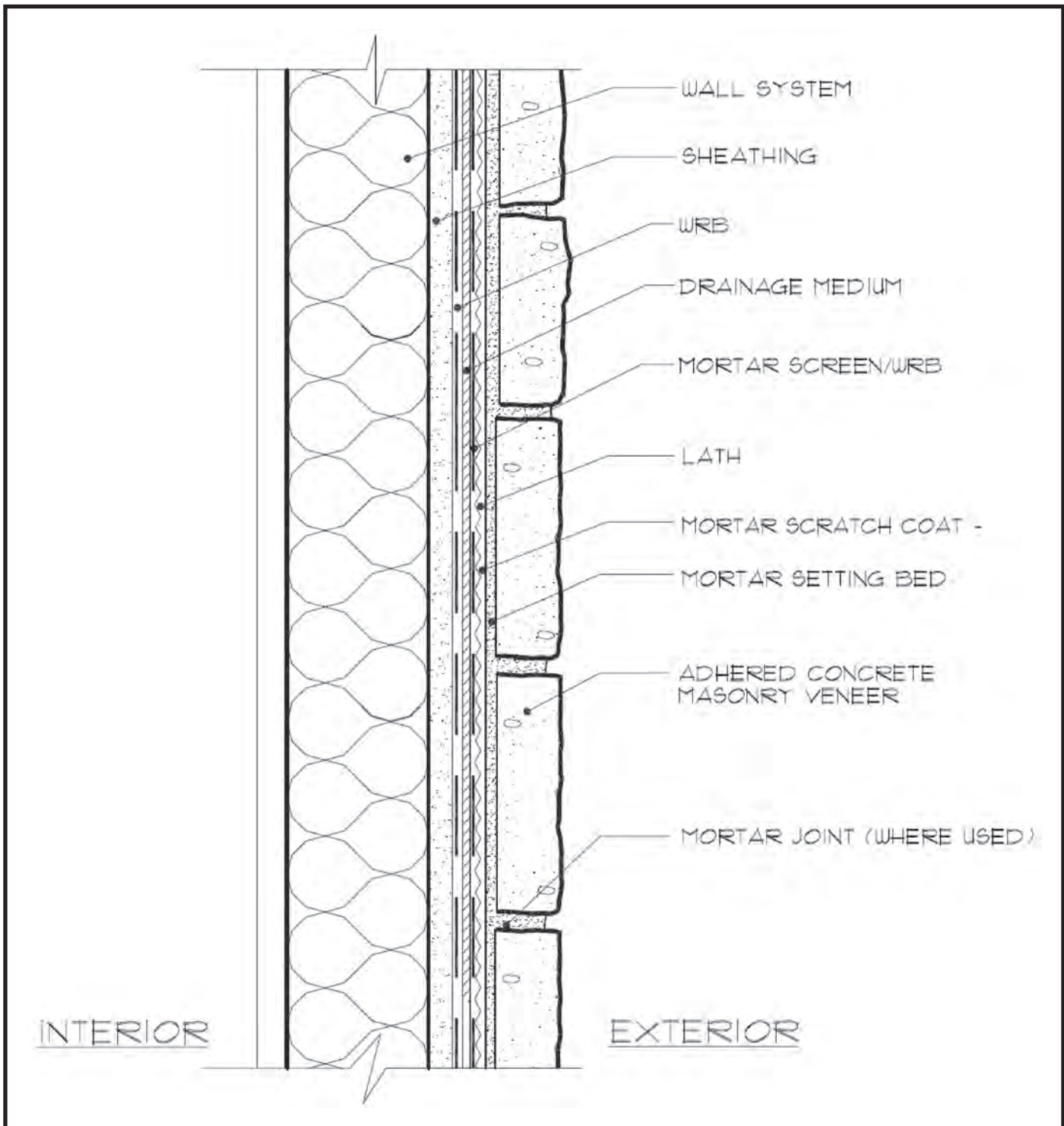
Fig. 35. Typical Wall Section - Optional Rainscreen System
