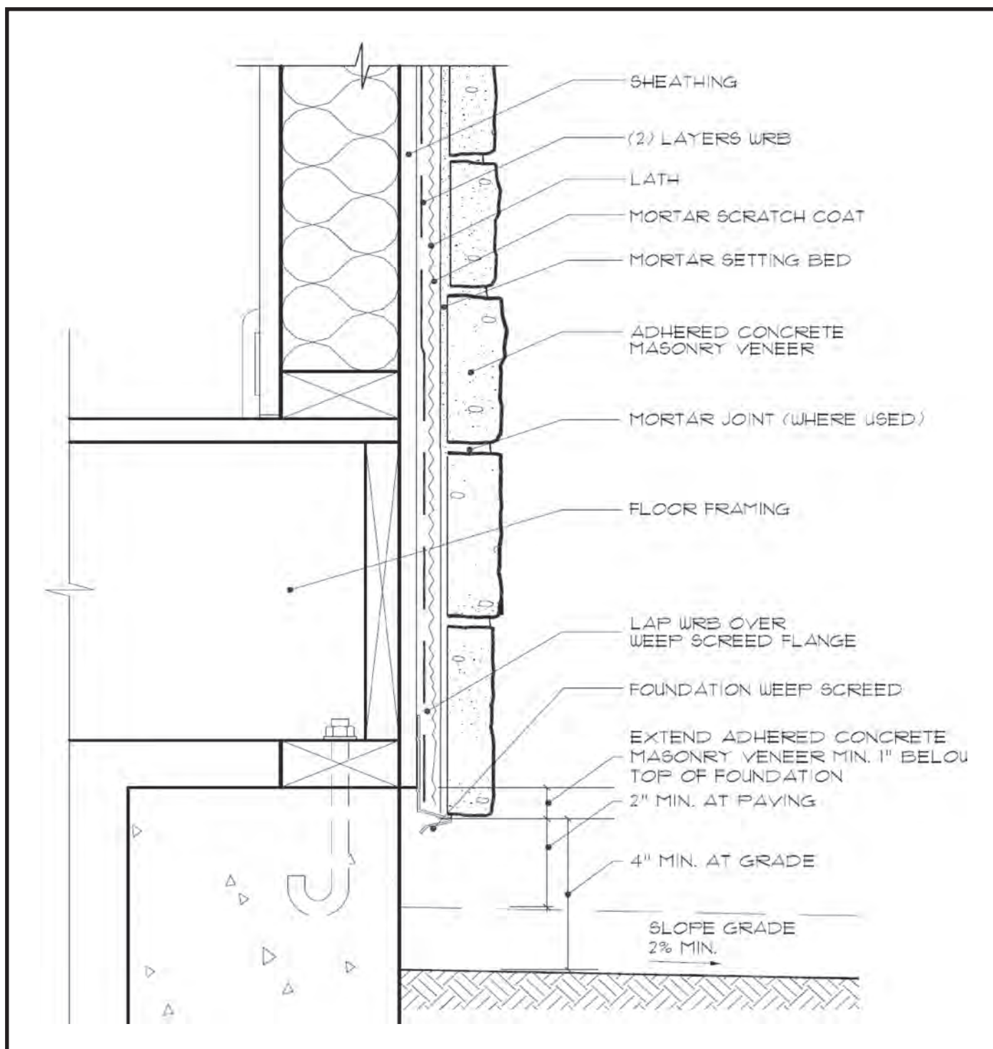
Fig. 3. Foundation Wall Base
