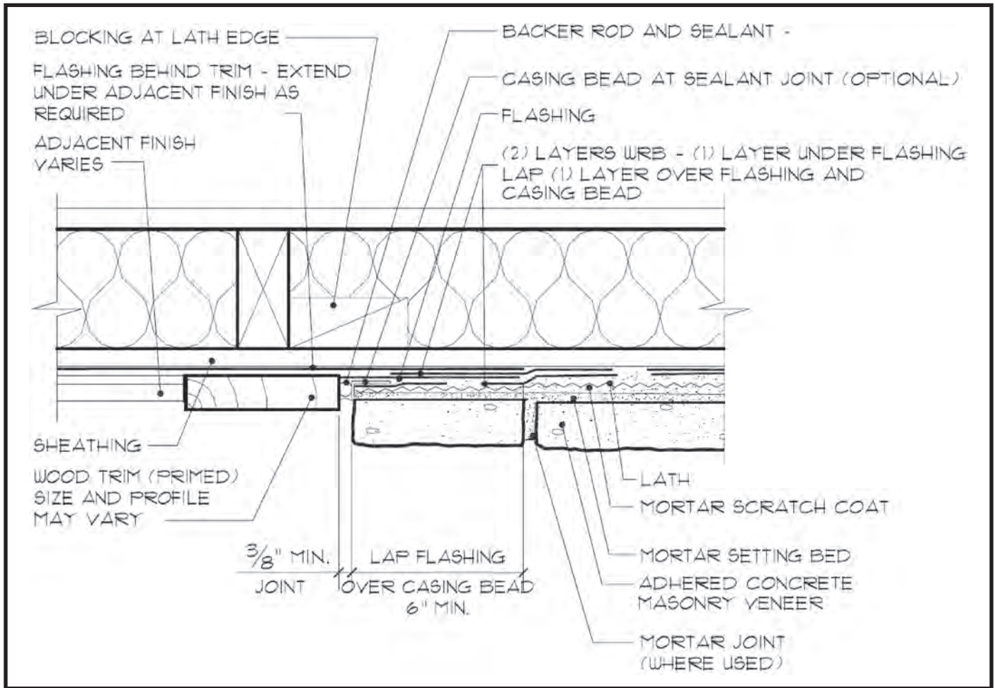
Fig. 10. Vertical Transition
