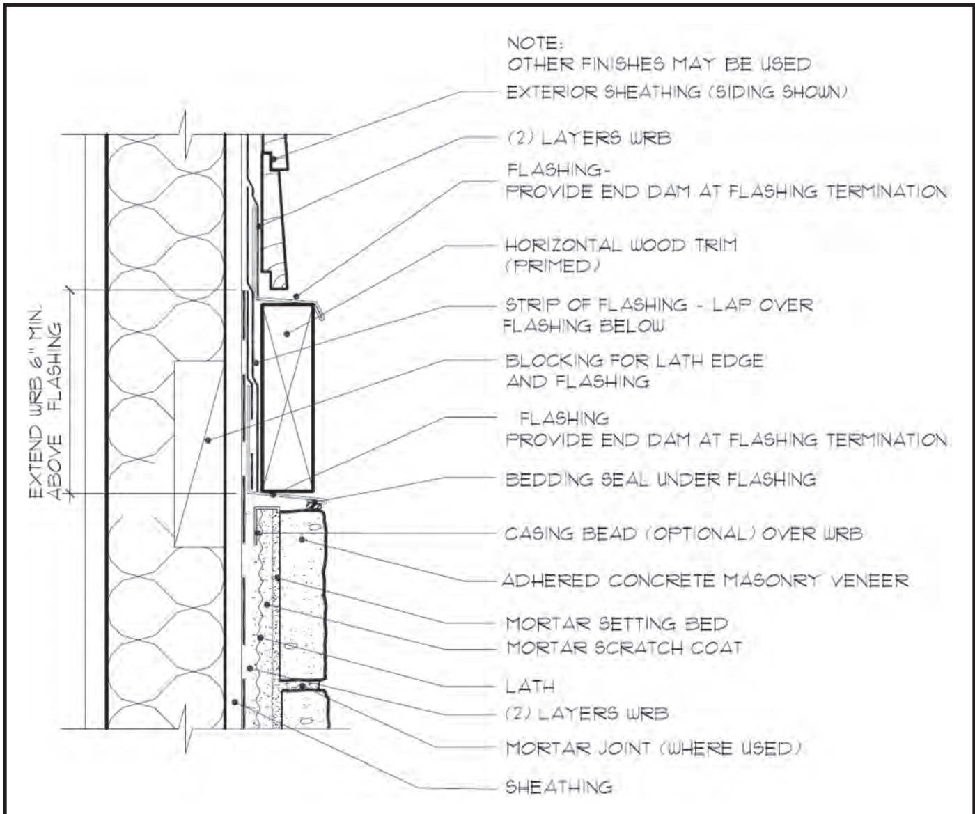
Fig. 9. Horizontal Transition
