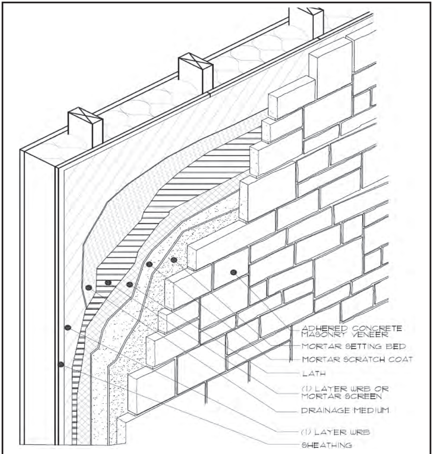
Fig. 32. Wall Assembly - Optional Rainscreen System - Drainage System
