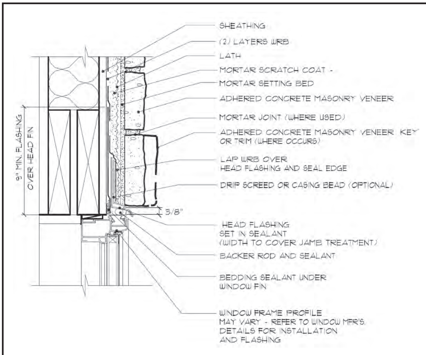
Fig. 21. Window Head
