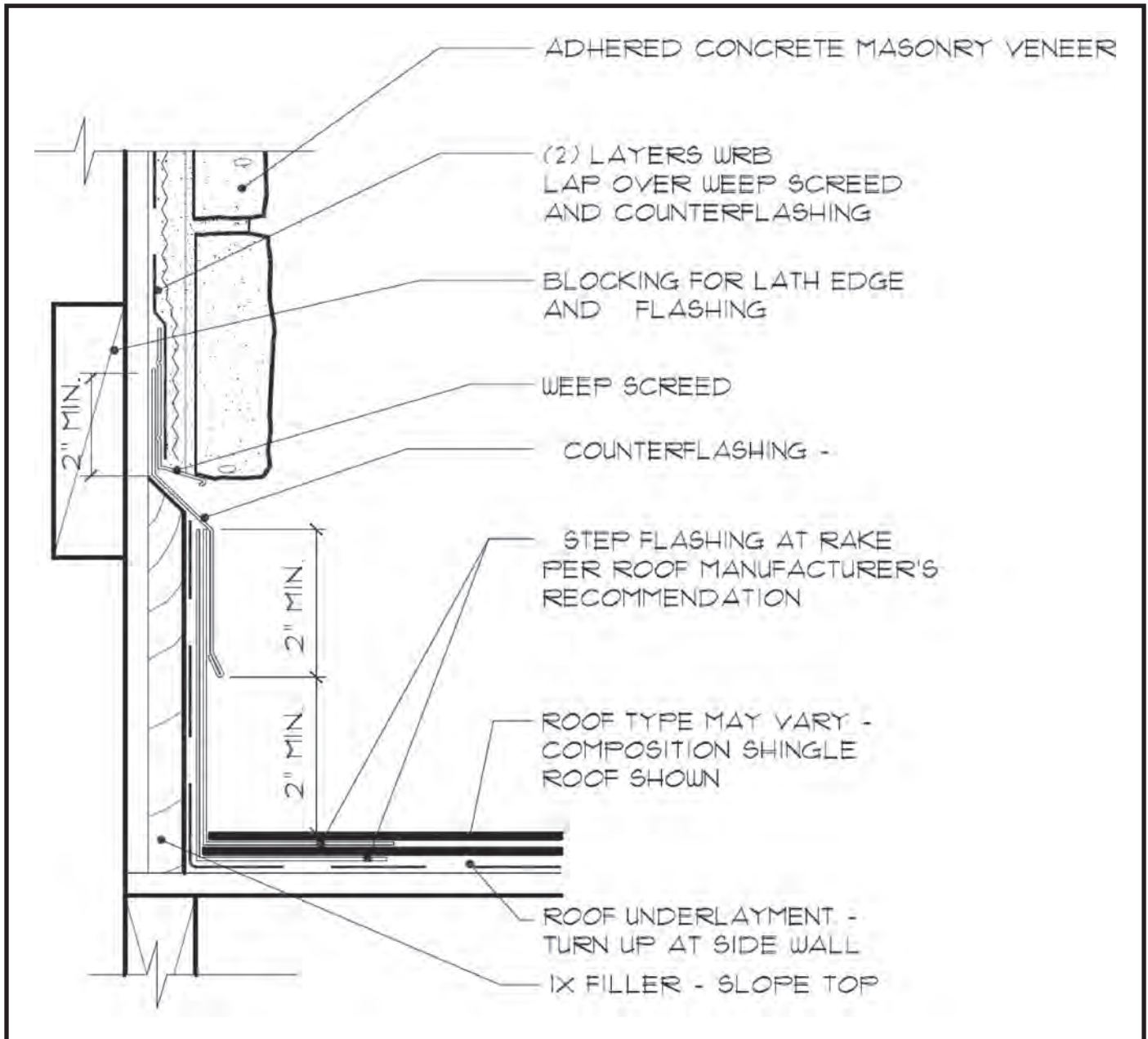
Fig. 16. Side Wall - Composition Shingles Curbing
