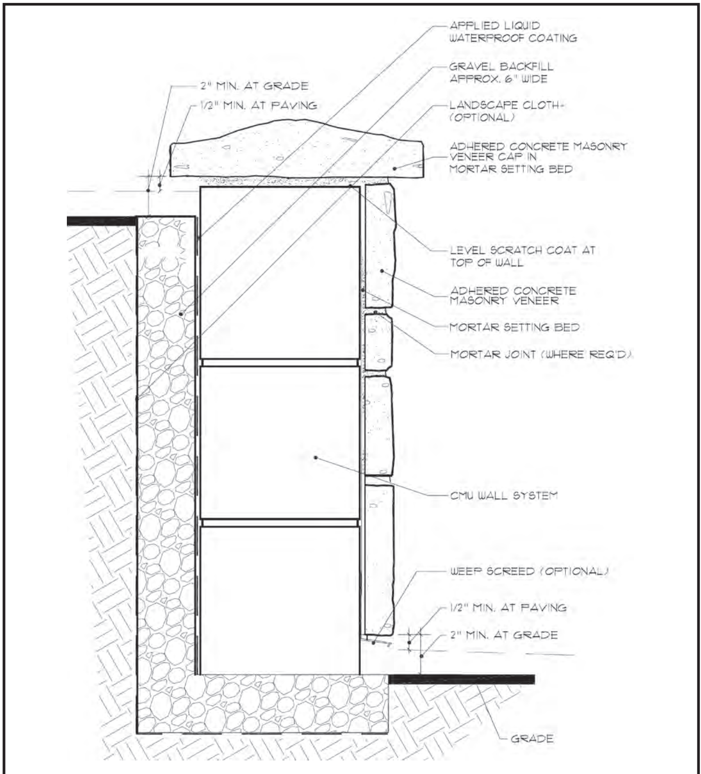
Fig. 36. Retaining Wall (CMU)
