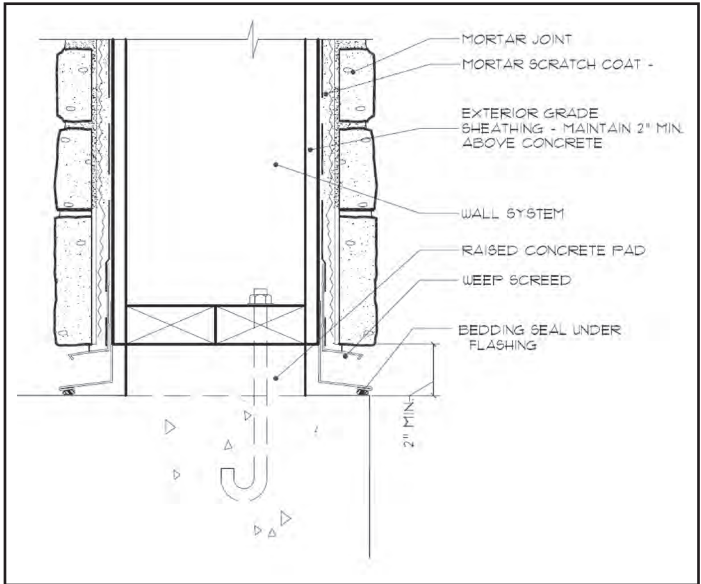
Fig. 26. Raised Column Base
