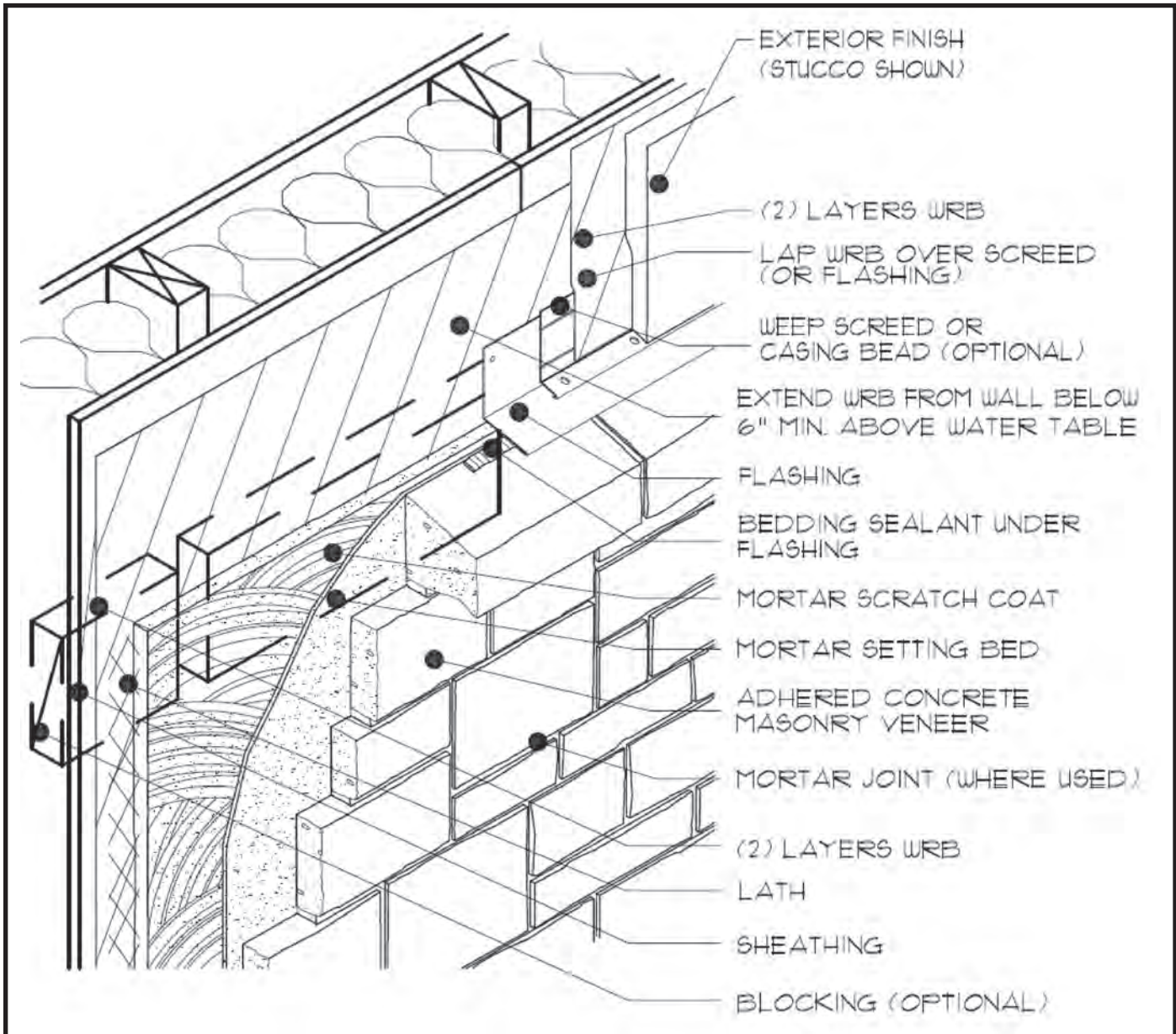
Fig. 1. Wall Assembly
