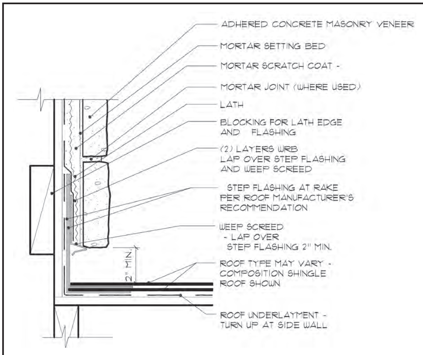
Fig. 15. Side Wall - Composition Shingles
