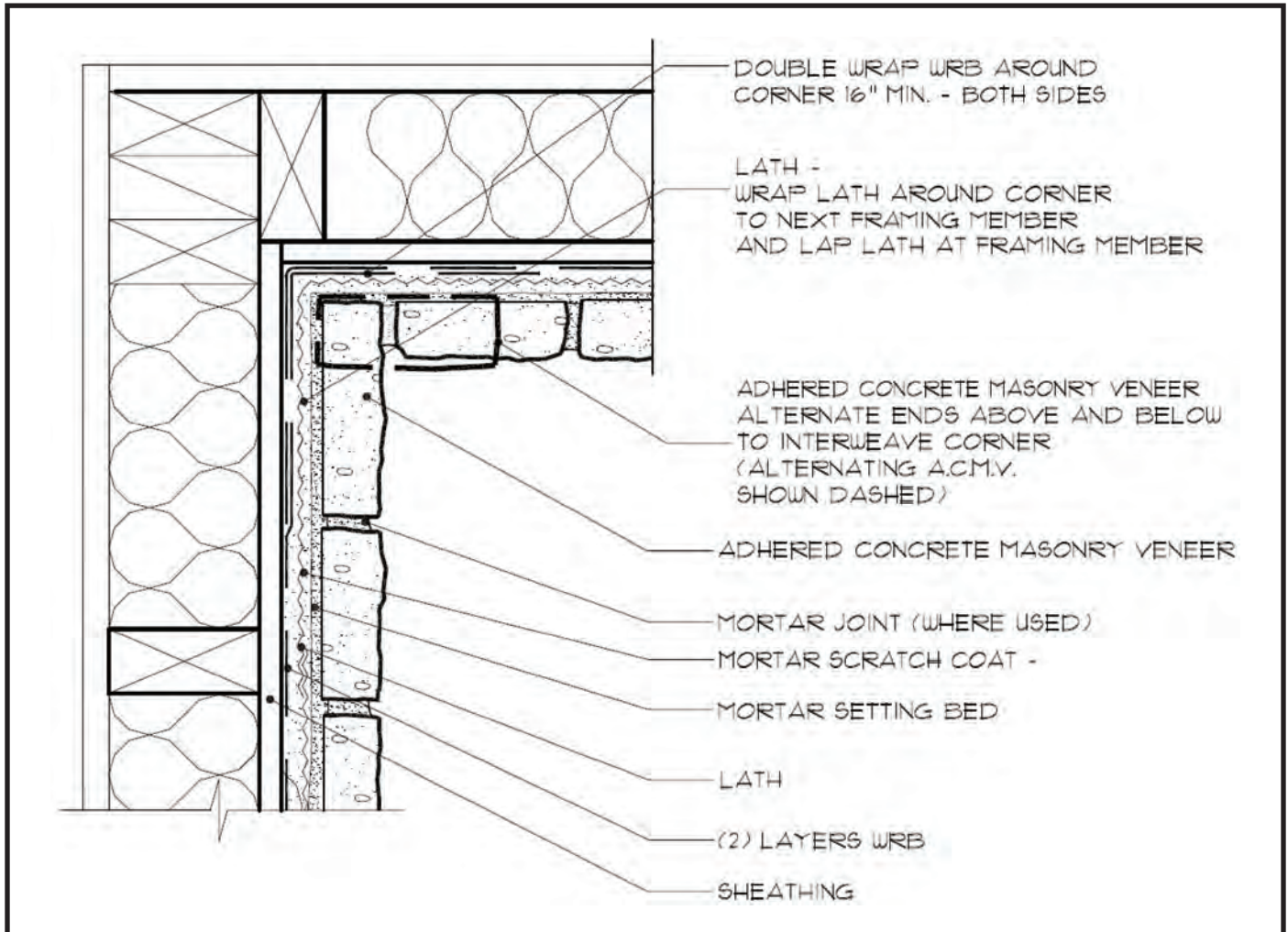
Fig. 8. Inside Corner
