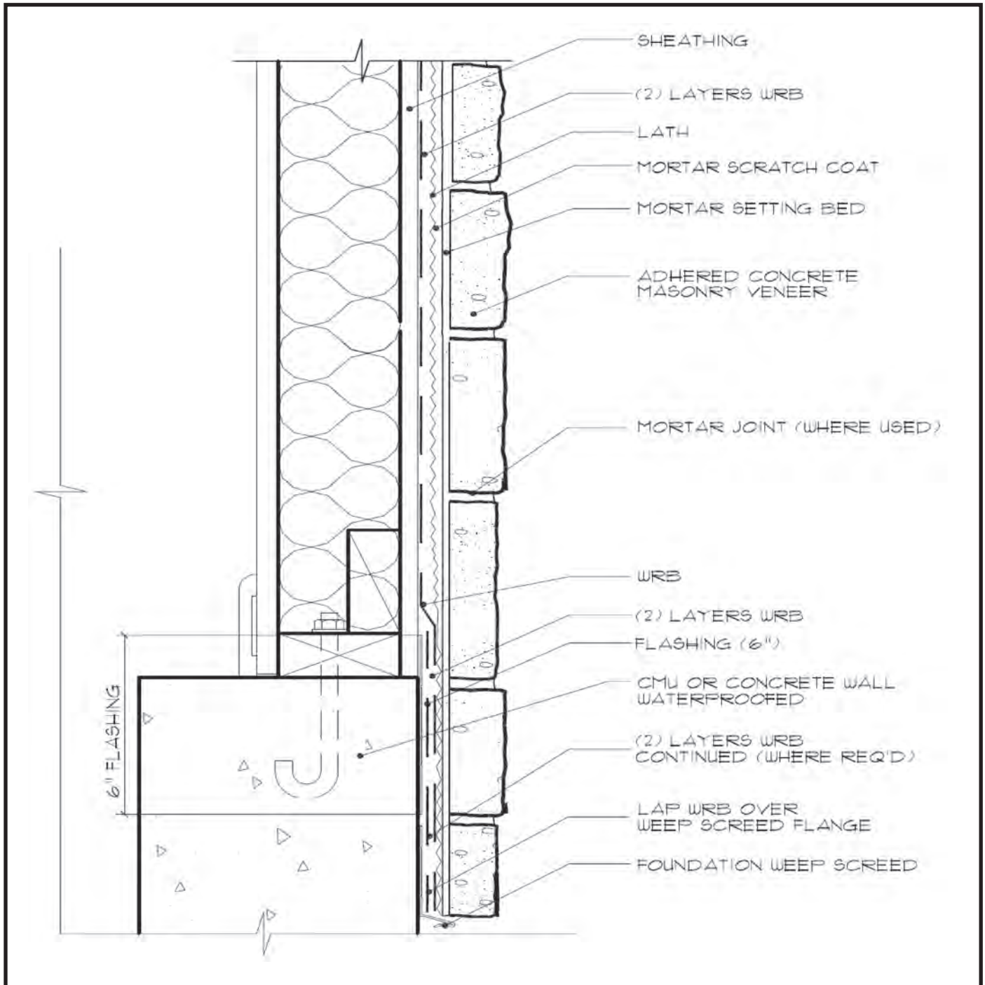
Fig. 4. Foundation Wall Base - ACMV Overlapping Foundation
