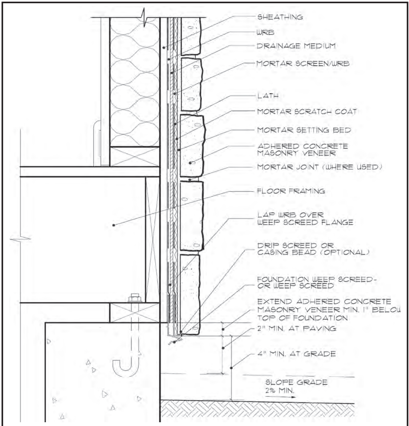
Fig. 34. Foundation Wall Base - Optional Rainscreen System
