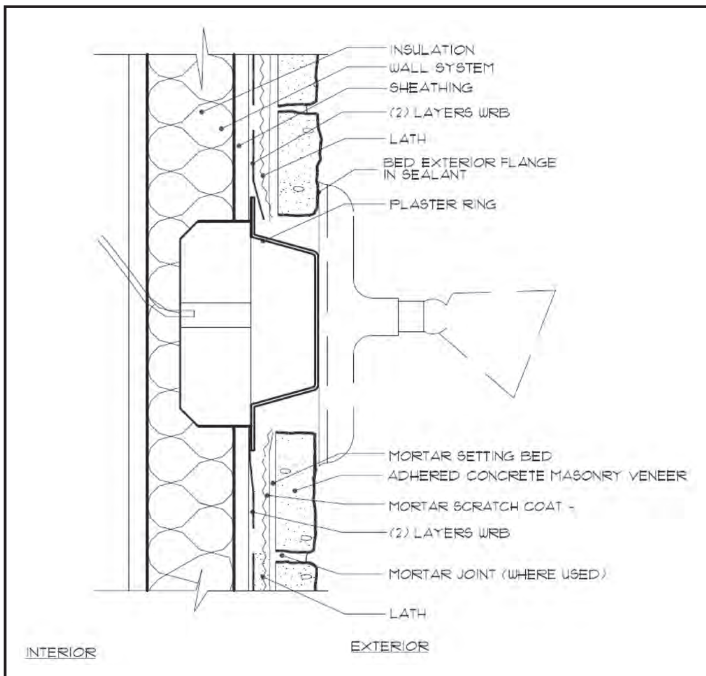
Fig. 27. Fixture Penetration
