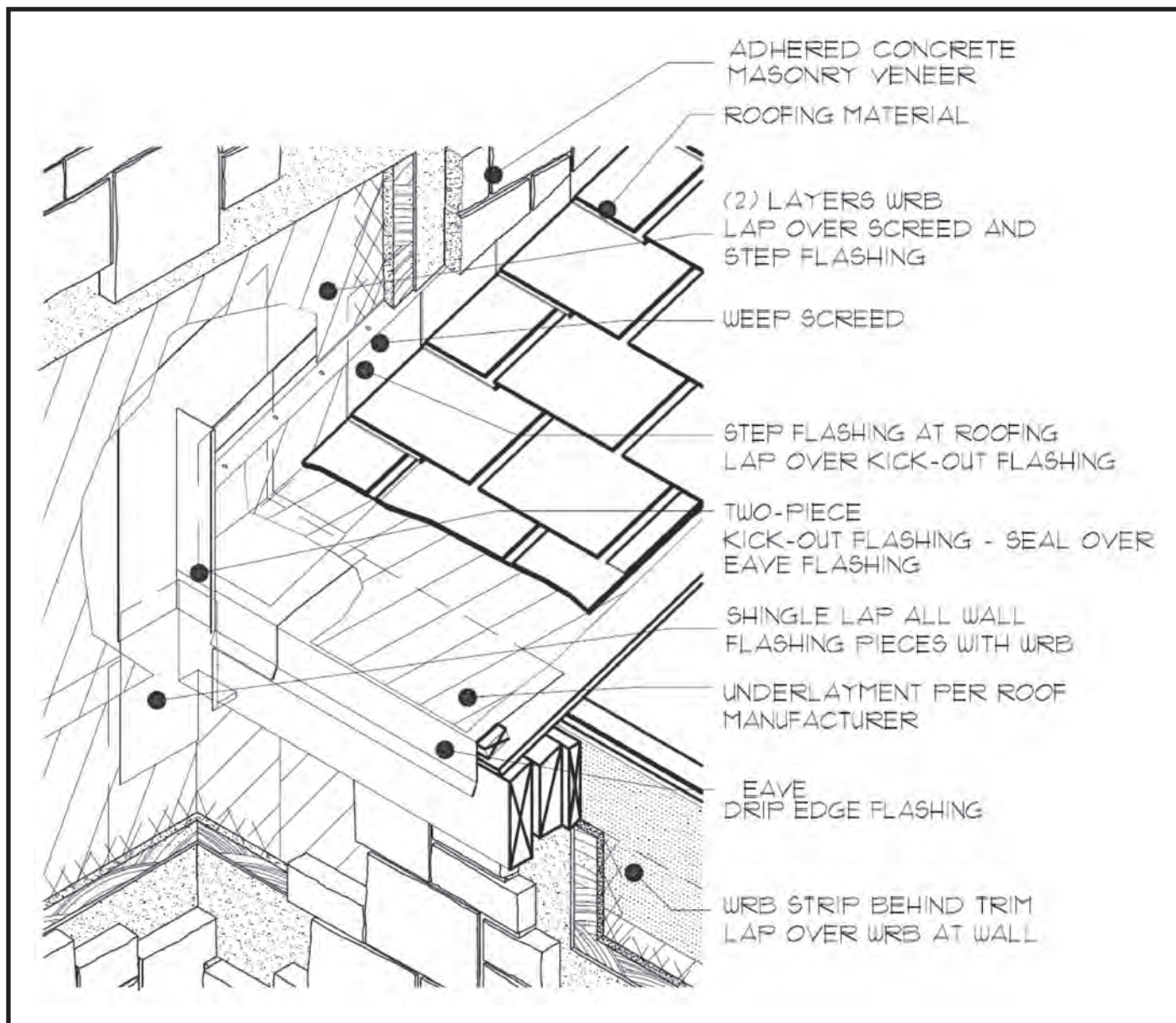
Fig. 22. Kick-Out Flashing
